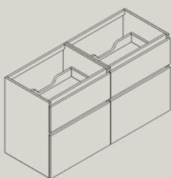
1200x460x650 mm (2x600 mm)
