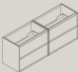
2000x460x600 mm (2x1000 mm)
