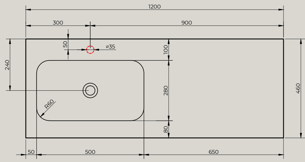
Top view
